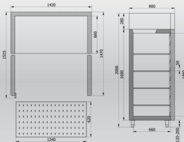
zamenljiva hladilna enota removable compact refrigerating unit
